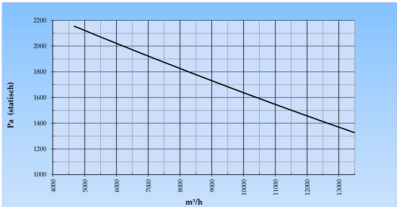
Curve TH 711A @ 1470rpm @ 15°C @ 0m
