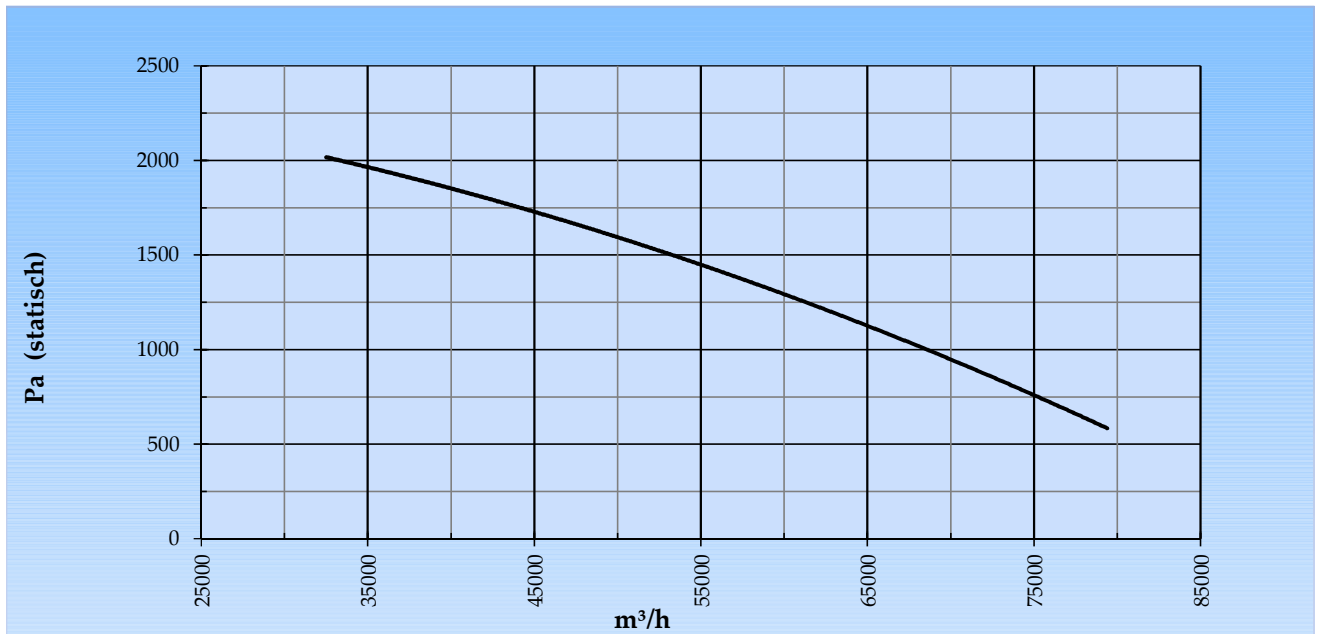
Curve BPR 1121D @ 985rpm @ 15°C @ 0m
