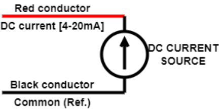
Figure 11 - DC current input
